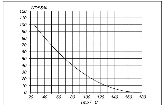
Fig. 15. Normalised avalanche energy rating. W_{DSS}\% = f(T_{mb}) ; conditions: I_D = 43 A
