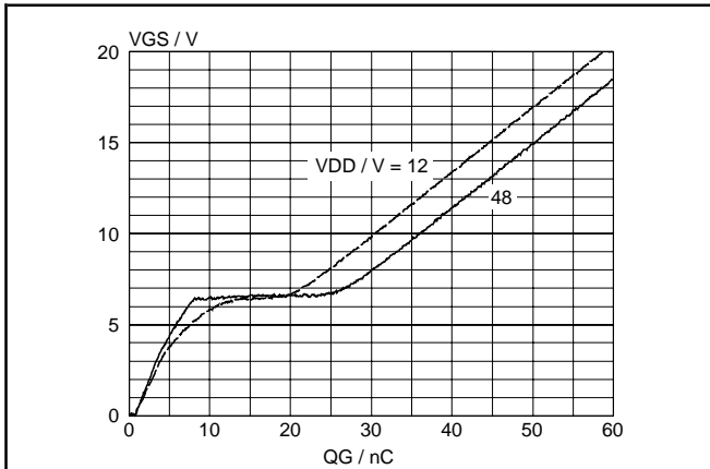
Fig. 13. Typical turn-on gate-charge characteristics. V_{GS} = f(Q_G) ; conditions: I_D = 43 A; parameter V_{DS}
